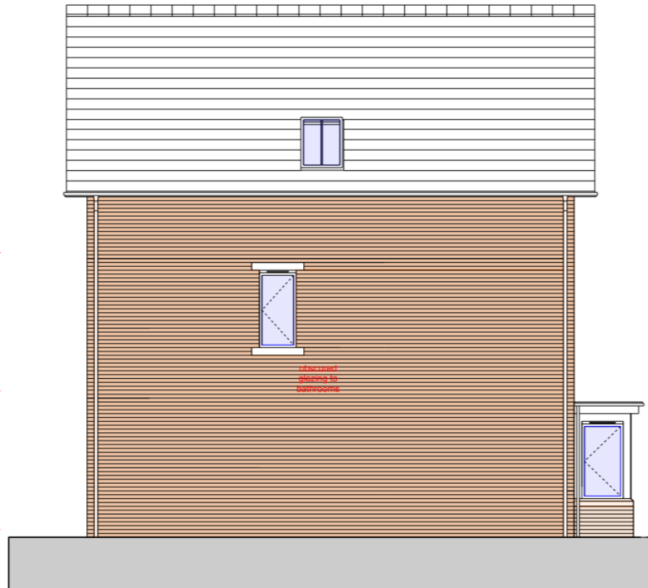
HOUSE ELEVATIONS Block One North
